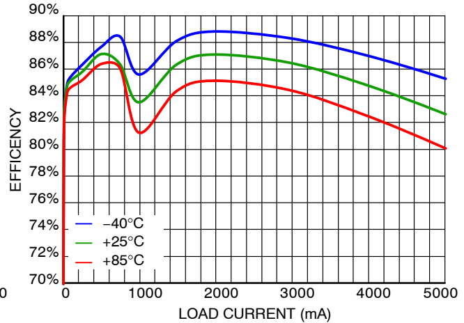
Figure 9. Efficiency vs. Load Current and Temperature, V_{IN} = 5\text{ V} , V_{OUT} = 1.2\text{ V}
