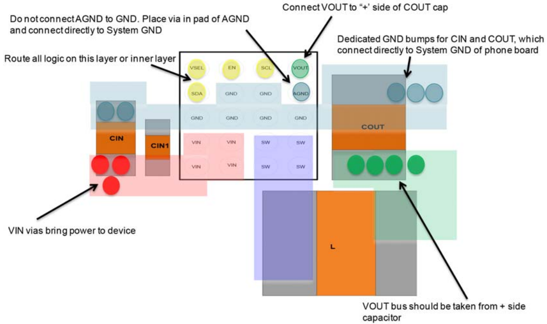
Figure 39. Guidance for Layer 1
