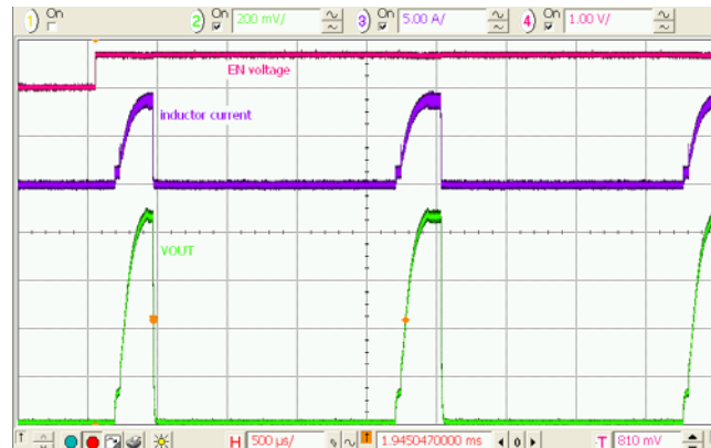
Figure 32. Startup into Faulted Load, V_{OUT}=0.9\text{ V}
