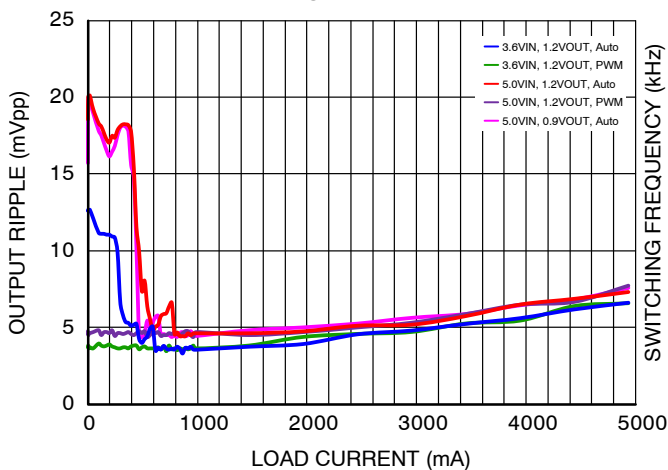
Figure 16. Output Ripple vs. Load Current, V_{IN} = 5\text{ V} and 3.6\text{ V} , V_{OUT} = 1.2\text{ V} and 0.9\text{ V} , Auto and FPWM
