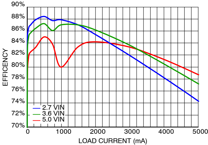
Figure 8. Efficiency vs. Load Current and Input Voltage, V_{OUT} = 0.9\text{ V}
