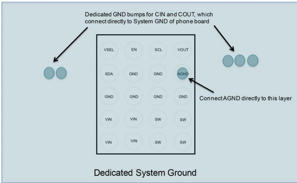
Figure 41. Guidance for Layer 3
