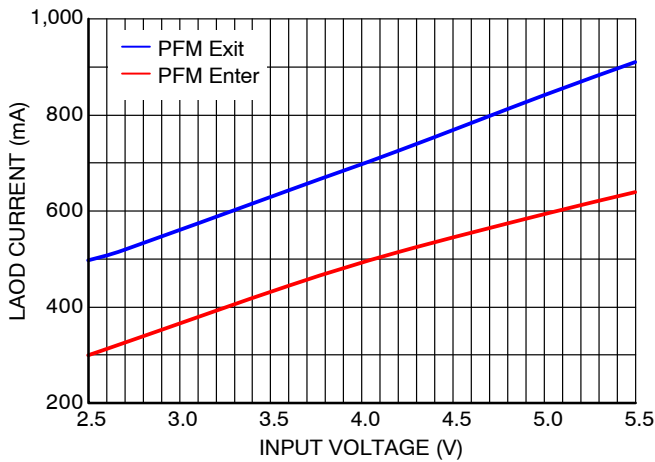
Figure 14. PFM Entry / Exit Level vs. Input Voltage, V_{OUT} = 1.2\text{ V}
