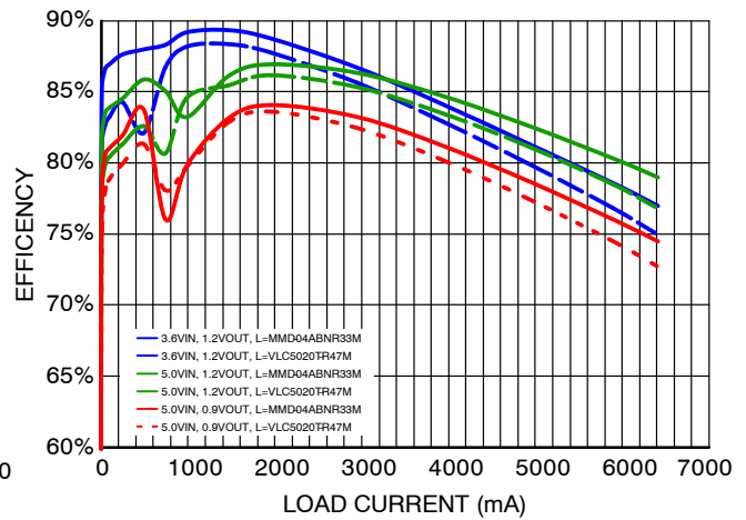
Figure 11. Efficiency vs. Load Current, V_{IN} = 3.6\text{ V} and 5\text{ V} , V_{OUT} = 1.2\text{ V} and 0.9\text{ V}
