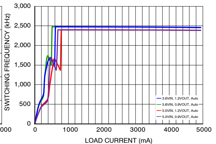
Figure 17. Frequency vs. Load Current, V_{IN} = 5\text{ V} and 3.6\text{ V} , V_{OUT} = 1.2\text{ V} and 0.9\text{ V} , Auto PWM
