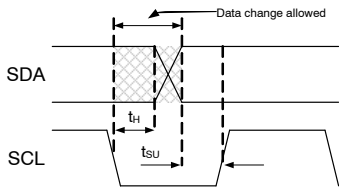
Figure 33. Data Transfer Timing
