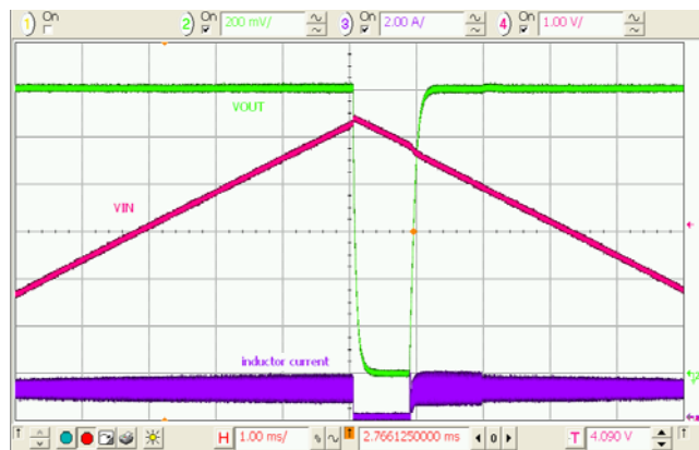
Figure 28. Input Over-Voltage Protection
