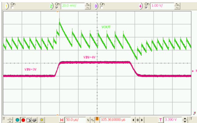
Figure 22. Line Transient, 3-4 V_{IN} , 1.2 V_{OUT} , 10 \mu\text{s} Edge, 50 \Omega Load
