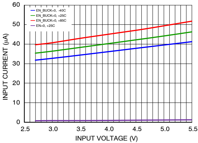
Figure 20. Shutdown Current vs. Input Voltage and Temperature
