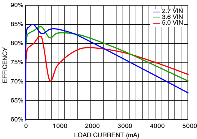
Figure 10. Efficiency vs. Load Current and Input Voltage, V_{OUT} = 0.6\text{ V}
