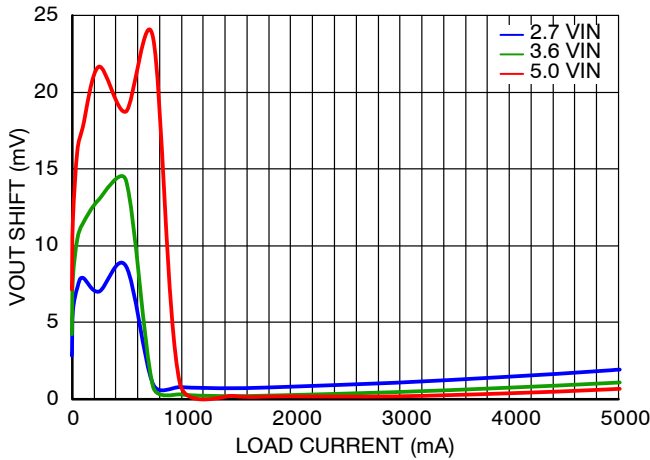
Figure 12. Output Regulation vs. Load Current and Input Voltage, V_{OUT} = 1.2\text{ V}
