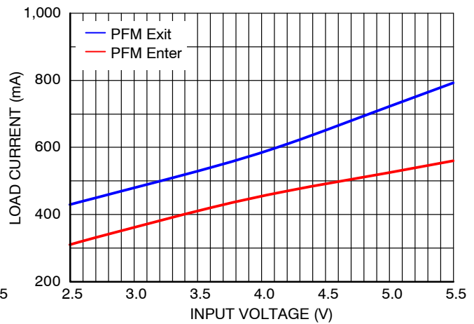
Figure 15. PFM Entry / Exit Level vs. Input Voltage, V_{OUT} = 0.9\text{ V}
