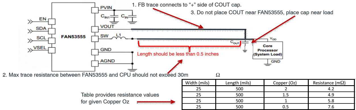
Figure 42. Remote Sensing Schematic
