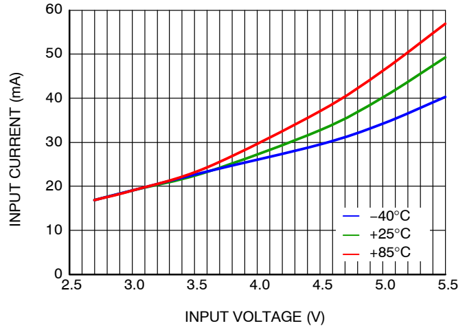
Figure 19. Quiescent Current vs. Input Voltage and Temperature, FPWM
