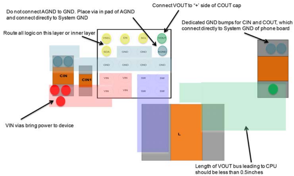
Figure 43. Remote Sensing Guidance, Top Layer
