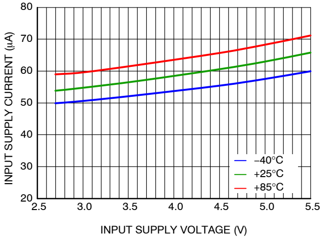
Figure 18. Quiescent Current vs. Input Voltage and Temperature, Auto PWM
