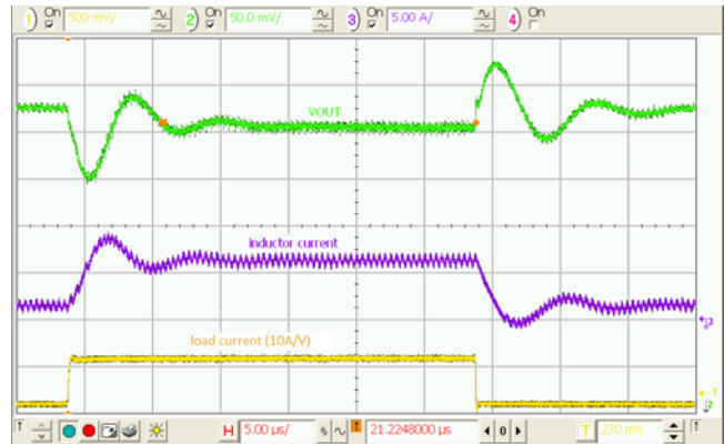
Figure 27. Load Transient, 3.6 V_{IN} , 1.2 V_{OUT} , 1.5–6 A, 100 ns Edge, C_{OUT}=4\times 22\ \mu\text{F}
