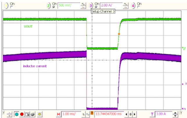
Figure 31. Overload Protection and Recovery
