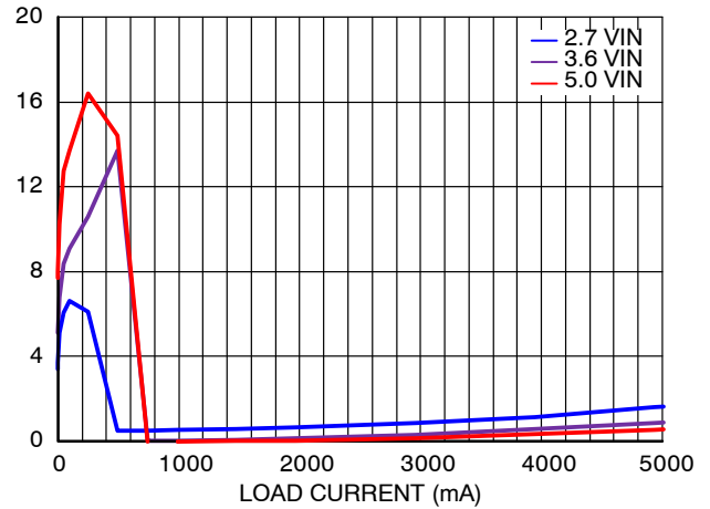
Figure 13. Output Regulation vs. Load Current and Input Voltage, V_{OUT} = 0.9\text{ V}
