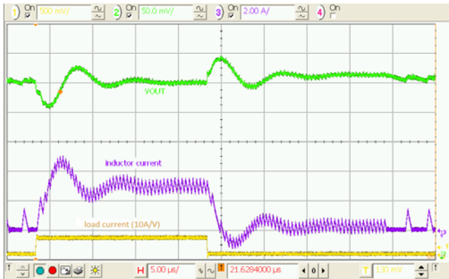
Figure 26. Load Transient, 3.6 V_{IN} , 1.2 V_{OUT} , 0.3–3 A, 100 ns Edge, C_{OUT}=4\times 22\ \mu\text{F}
