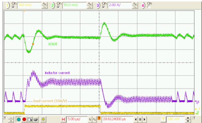
Figure 25. Load Transient, 3.6 V_{IN} , 1.2 V_{OUT} , 0.3–3 A, 100 ns Edge
