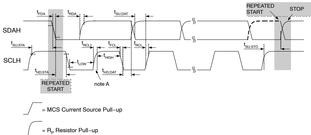
Figure 5. I 2 C Interface Timing for High-Speed Mode
