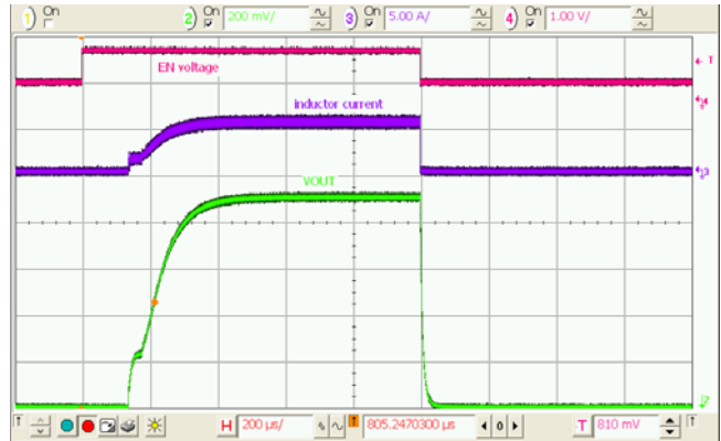
Figure 30. Startup / Shutdown, 180 mΩ Load, V_{OUT}=0.9\text{ V}
