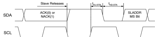
Figure 36. REPEATED START Timing
