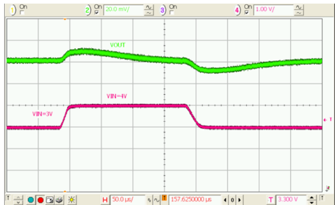
Figure 23. Line Transient, 3-4 V_{IN} , 1.2 V_{OUT} , 10 \mu\text{s} Edge, 1 A Load
