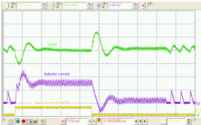
Figure 24. Load Transient, 5 V_{IN} , 0.9 V_{OUT} , 0.3–3 A, 100 ns Edge
