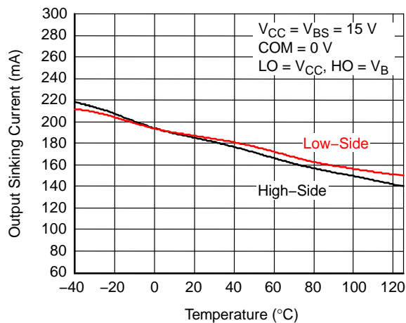
Figure 17. Output Sinking Current vs. Temperature
