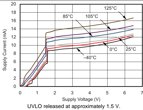
Figure 6. TPS386000-Q1 Supply Current vs Supply Voltage
