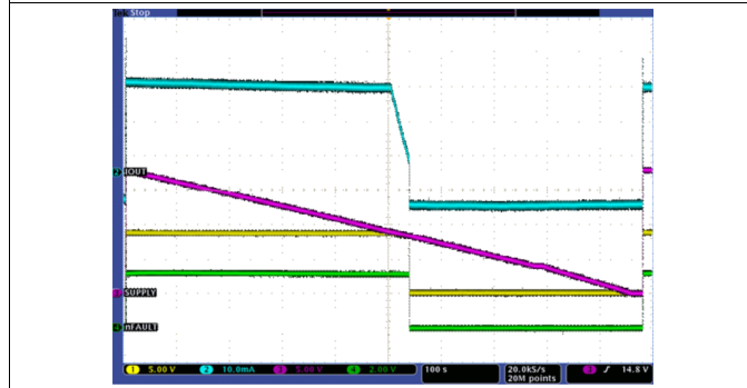
Figure 21. Transient Overvoltage (16 V – 18 V – 17 V – 16 V)
