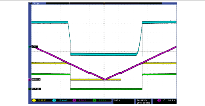
Figure 22. Transient Undervoltage (10.8 V – 9 V – 10.8 V)
