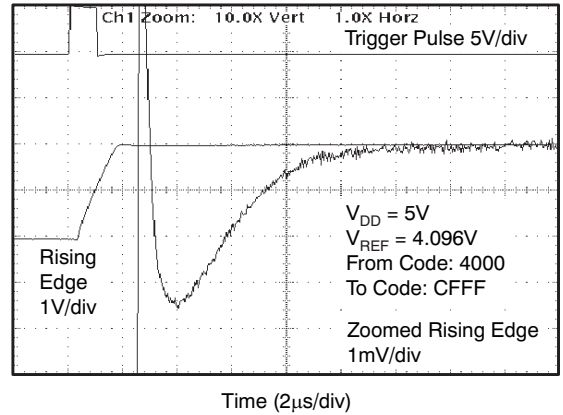
Figure 15. Half-Scale Settling Time, 5-V Rising Edge
