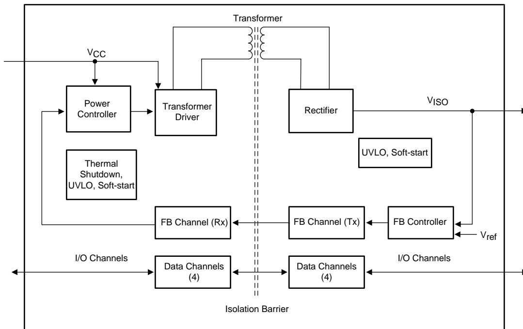
Figure 34. Block Diagram
