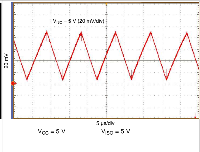
Figure 30. V_{ISO} Ripple Voltage at 130 mA
