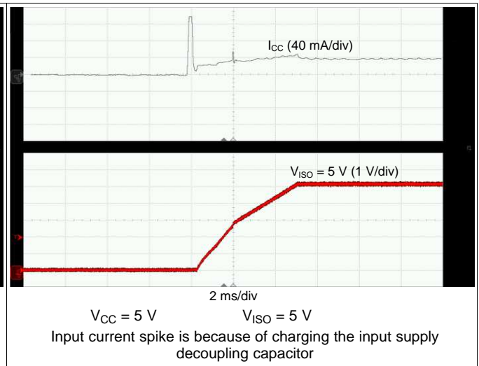
Figure 28. Soft Start at 10-mA Load
