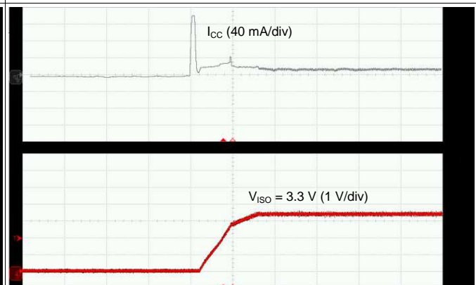
Figure 26. Soft Start at 10-mA Load
