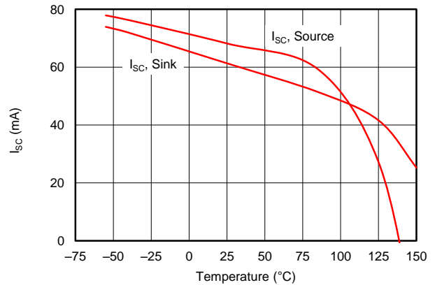
Figure 44. Short-Circuit Current vs Temperature
