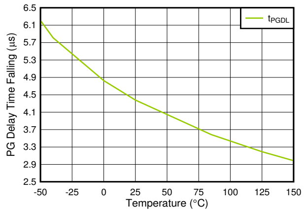
Figure 6-26. t_{PGDL} vs Temperature
