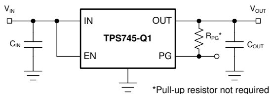
Typical Application: Fixed Voltage Version
