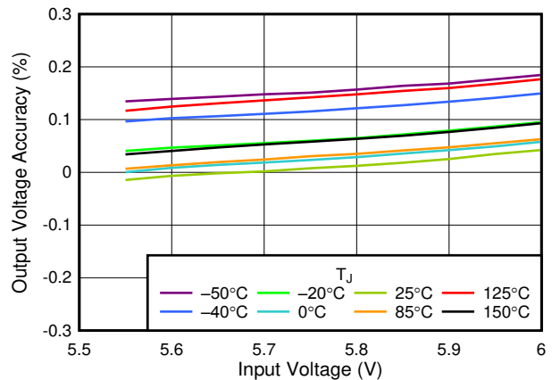
Figure 6-8. 5.5-V Line Regulation vs V_{IN}
