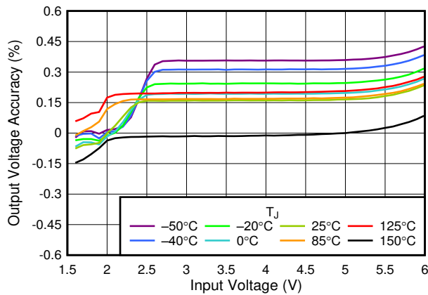
Figure 6-7. 0.55-V Line Regulation vs V_{IN}
