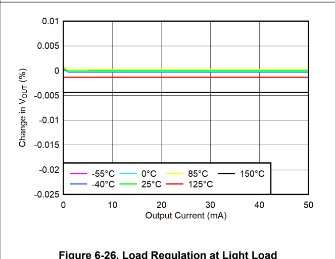
Figure 6-26. Load Regulation at Light Load
