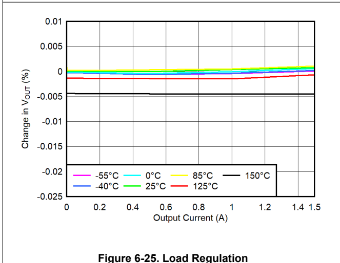
Figure 6-25. Load Regulation
