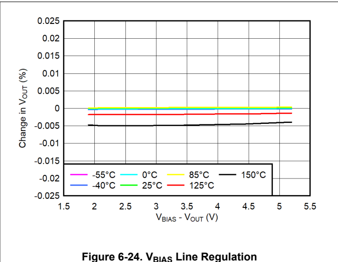
Figure 6-24. V_{BIAS} Line Regulation
